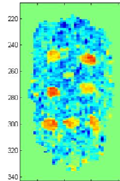
HYPERSPECTRAL IMAGE
