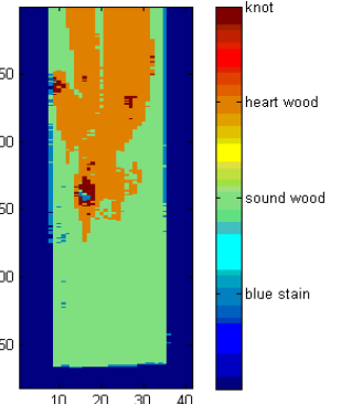
CLASSIFICATION
